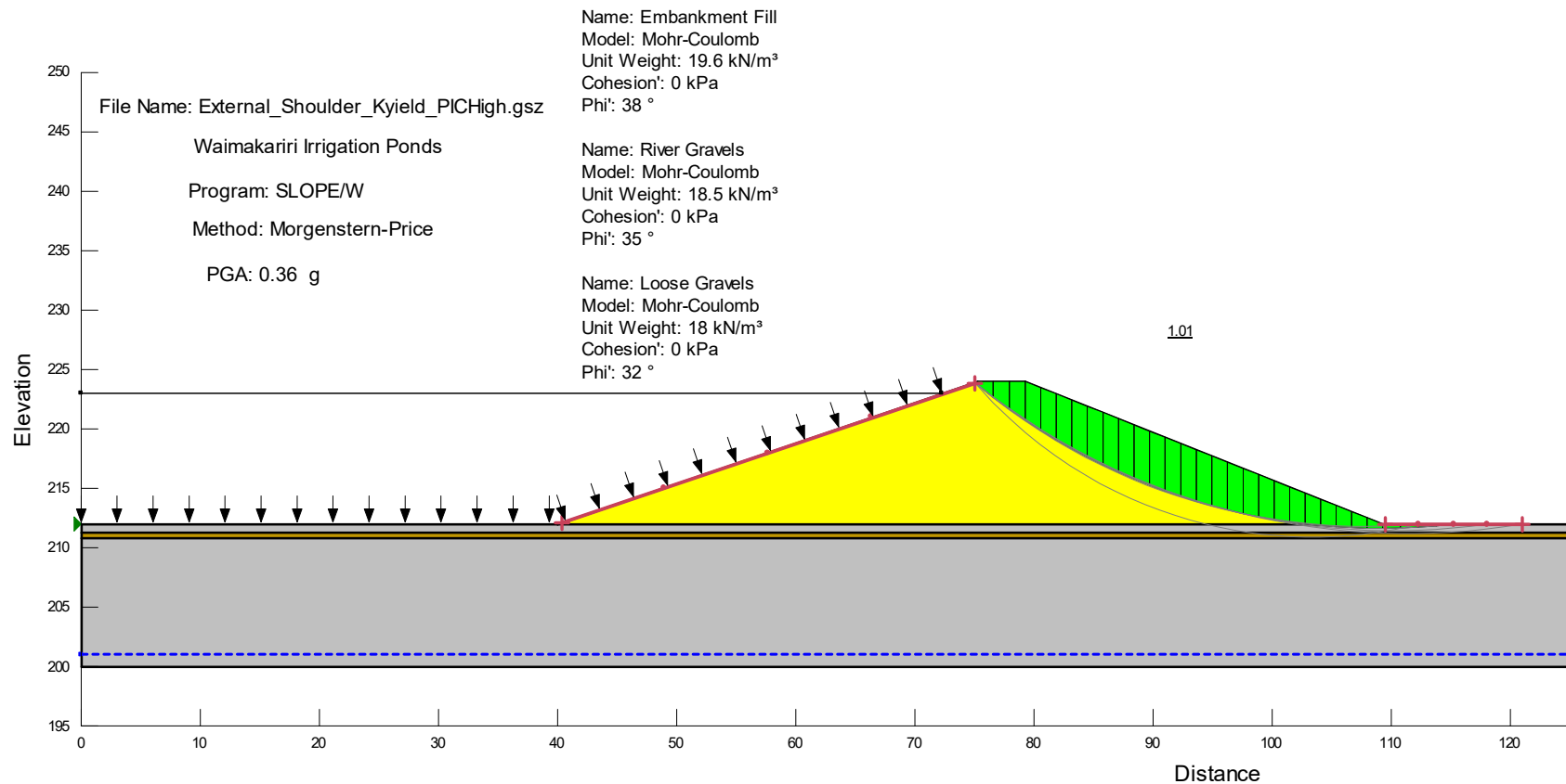
Figure D12 - Pseudo-Static at Yield Acceleration: External Downstream Shoulder (High PIC)
