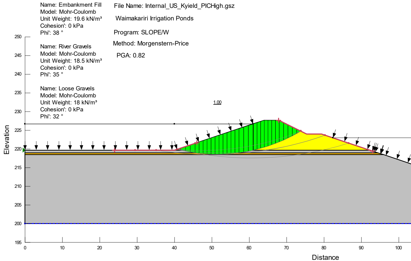
Figure D10 - Pseudo-Static at Yield Acceleration: Internal Upstream Shoulder (High PIC)
