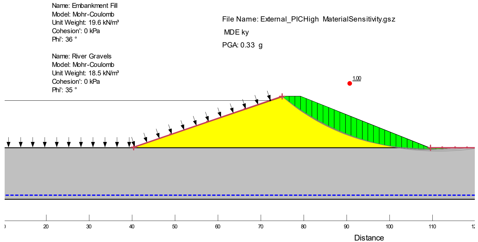
Figure D20 – Pseudo-Static with \phi' = 36^\circ at Yield Acceleration: External Downstream Shoulder (High PIC)
