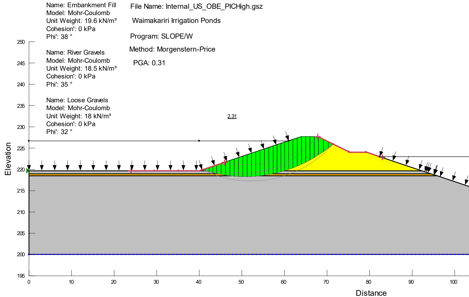
Figure D6 – Pseudo-Static at OBE with No Seepage: Internal Upstream Shoulder (High PIC)
