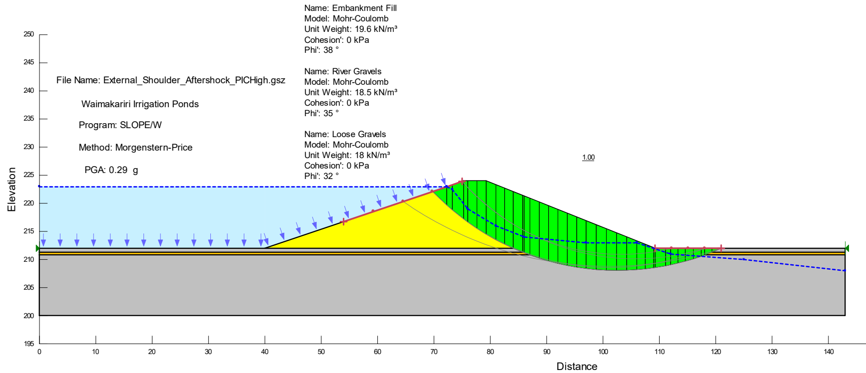
Figure D16 – Post-Seismic Aftershock Yield Acceleration with Seepage: External Upstream Shoulder (High PIC)
