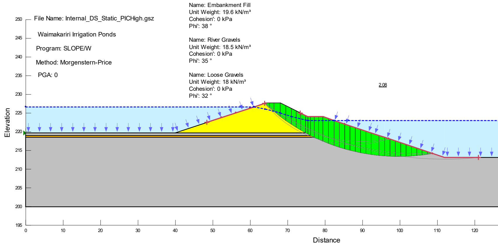
Figure D3 – Static Stability with Steady State Seepage: Internal Downstream Shoulder (High PIC)
