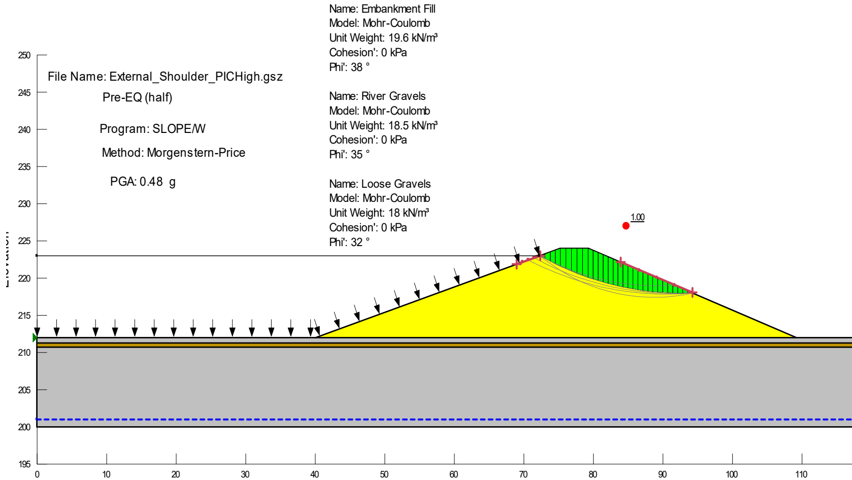
Figure D22 - Pseudo-Static at Yield Acceleration within Upper Half: External Downstream Shoulder (High PIC)
