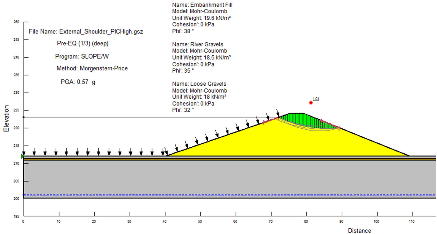
Figure D23 - Pseudo-Static at Yield Acceleration within Upper Third: External Downstream Shoulder (High PIC)
