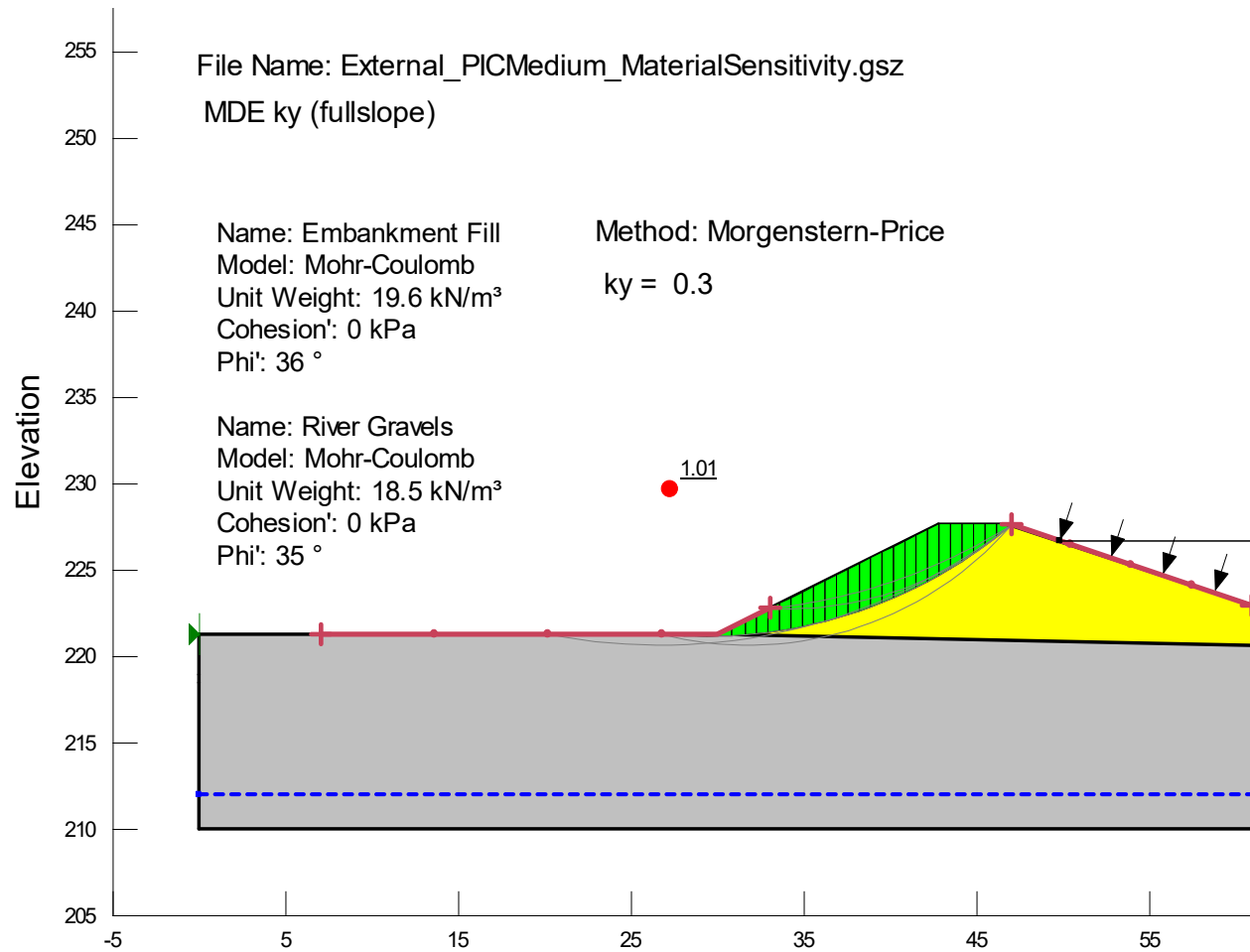
Figure D19 – Pseudo-Static with \phi' = 36^\circ at Yield Acceleration: External Downstream Shoulder (Medium PIC)
