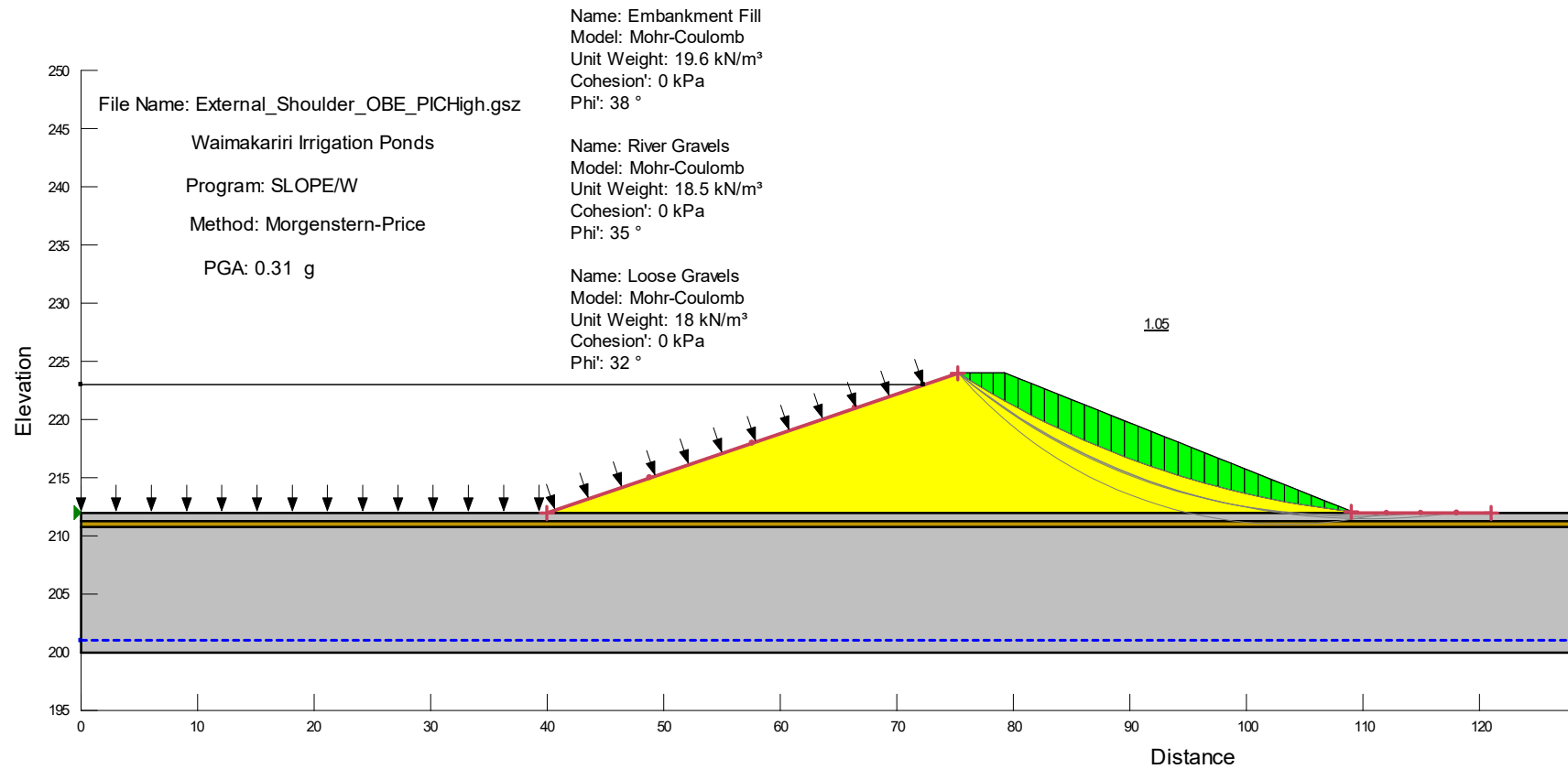
Figure D8 – Pseudo-Static at OBE with No Seepage: External Downstream Shoulder (High PIC)
