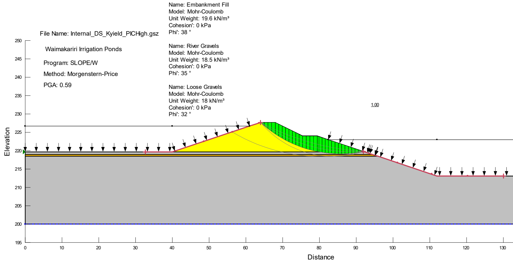
Figure D11 - Pseudo-Static at Yield Acceleration: Internal Downstream Shoulder (High PIC)
