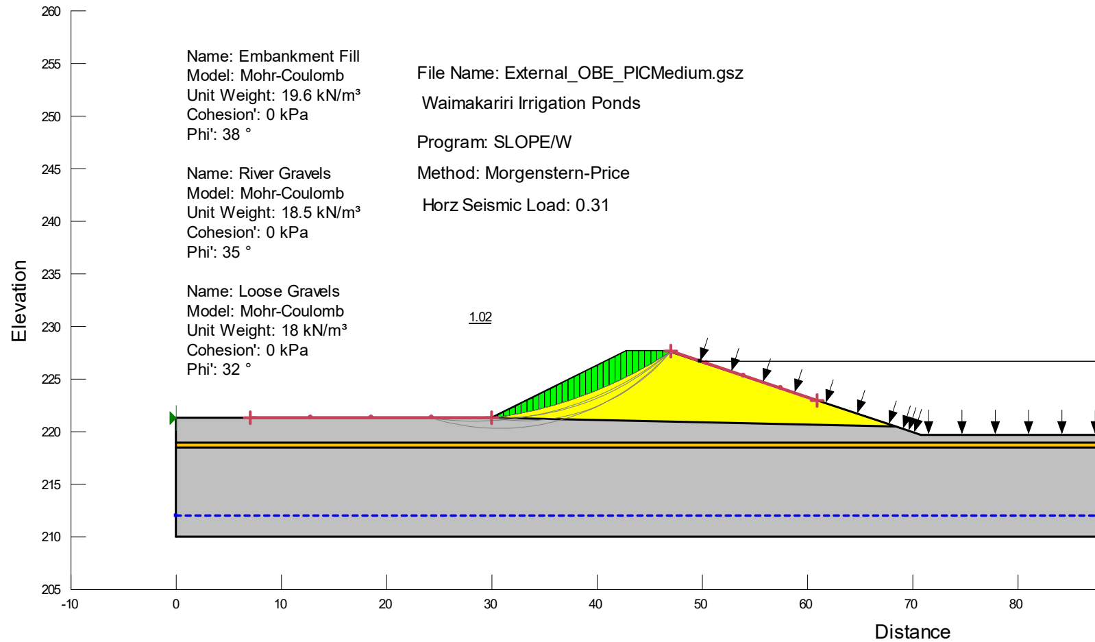
Figure D5 – Pseudo-Static at OBE with No Seepage: External Downstream Shoulder (Medium PIC)
