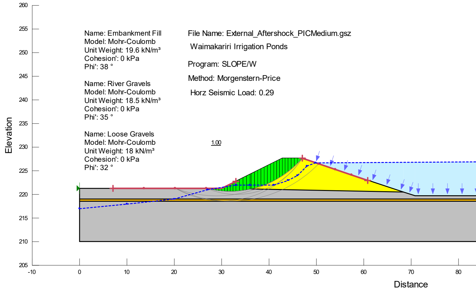
Figure D13 – Post-Seismic Aftershock Yield Acceleration with Seepage: External Upstream Shoulder (Medium PIC)
