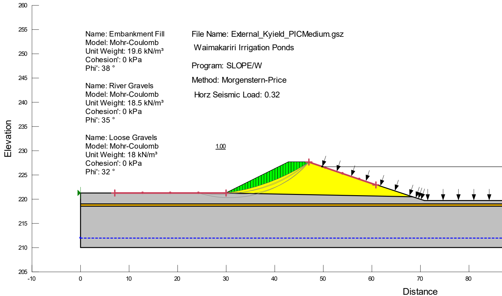
Figure D9 - Pseudo-Static at Yield Acceleration: External Downstream Shoulder (Medium PIC)
