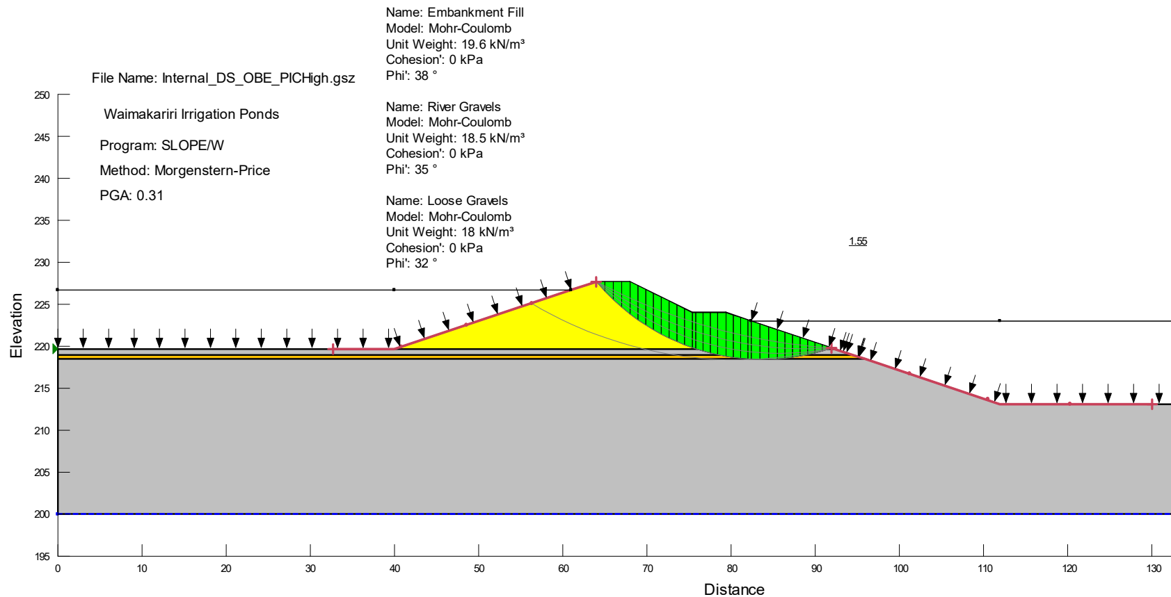
Figure D7 – Pseudo-Static at OBE with No Seepage: Internal Downstream Shoulder (High PIC)
