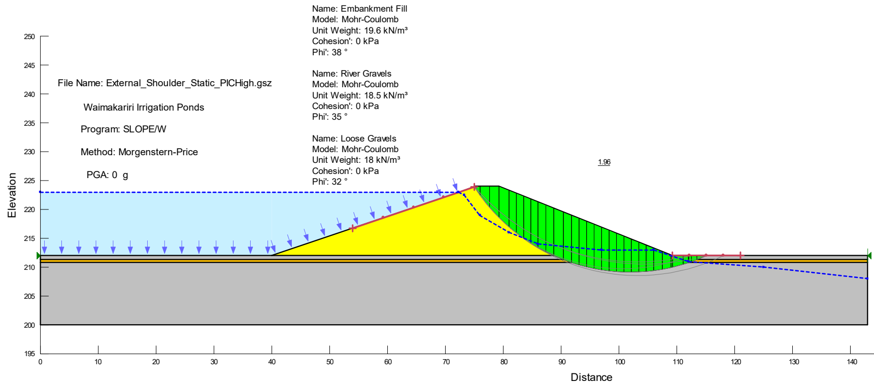
Figure D4 – Static Stability with Steady State Seepage: External Downstream Shoulder (High PIC)
