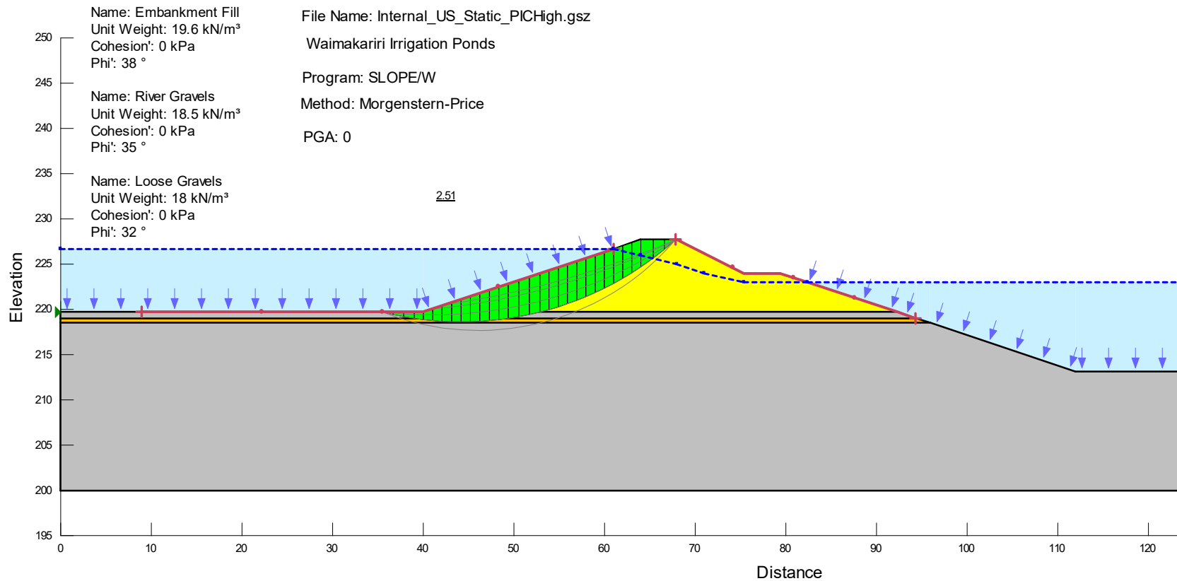
Figure D2 – Static Stability with Steady State Seepage: Internal Upstream Shoulder (High PIC)
