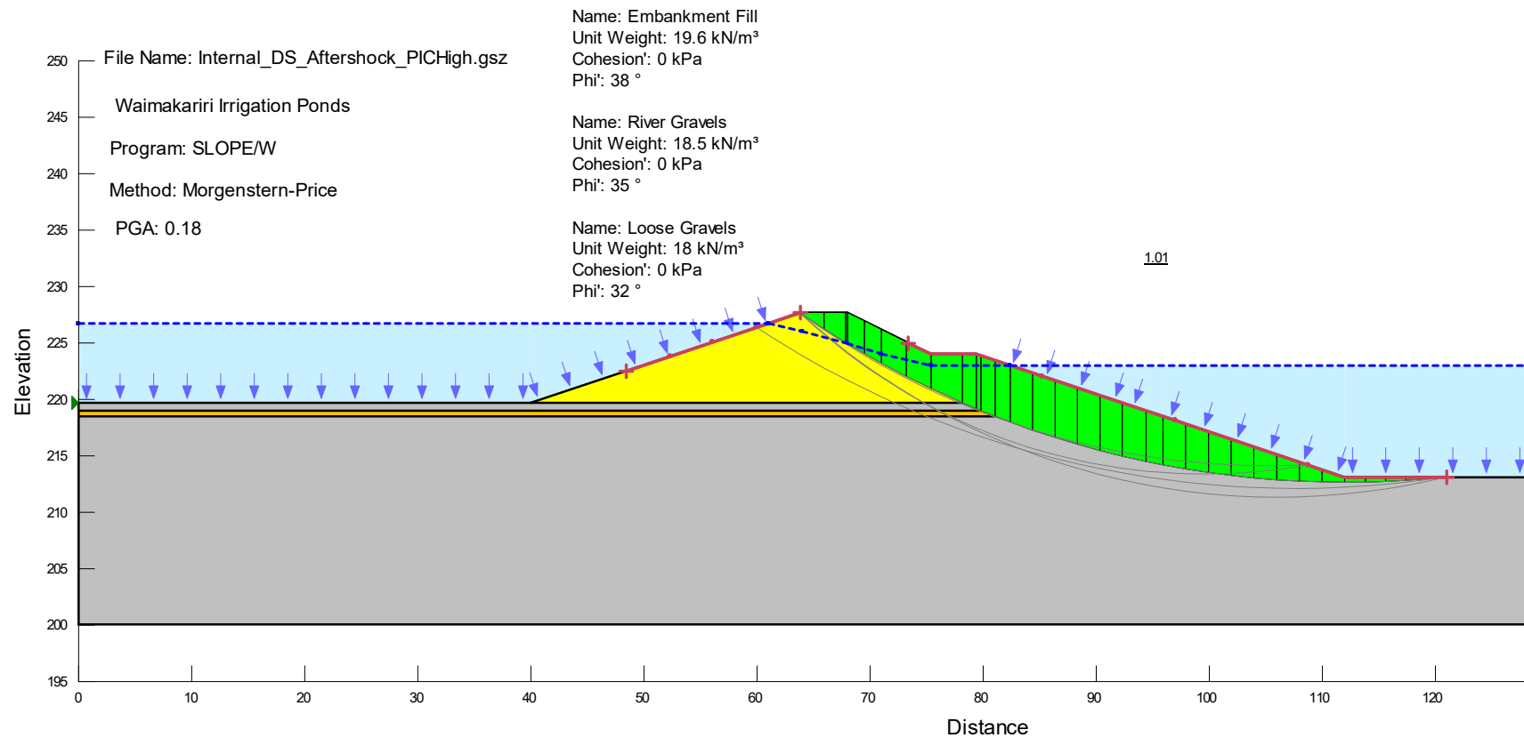
Figure D15 – Post-Seismic Aftershock Yield Acceleration with Seepage: Internal Downstream Shoulder (High PIC)
