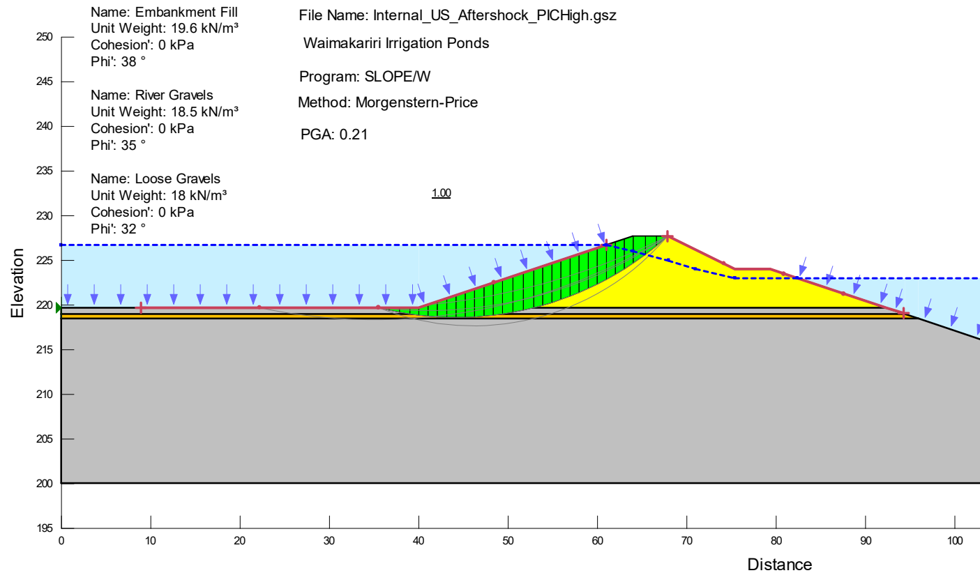
Figure D14 – Post-Seismic Aftershock Yield Acceleration with Seepage: Internal Upstream Shoulder (High PIC)
