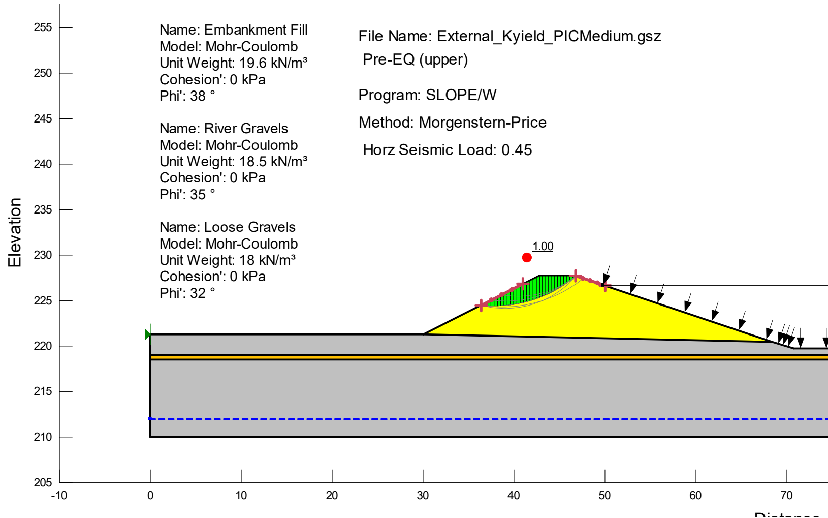
Figure D21 - Pseudo-Static at Yield Acceleration within Upper Half: External Downstream Shoulder (Medium PIC)
