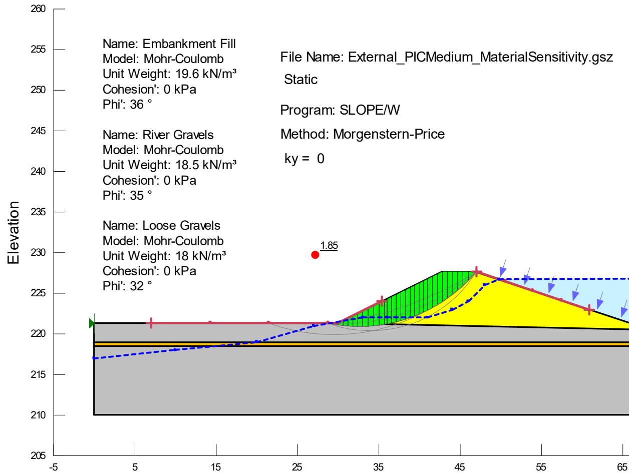
Figure D17 – Static Stability with \phi' = 36^\circ and Steady State Seepage: External Downstream Shoulder (Medium PIC)
